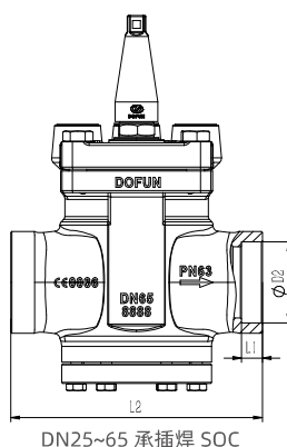
先导主阀 Pilot Main Valve
